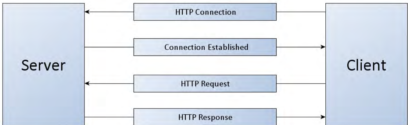
Figure 2 – HTTP Protocol
